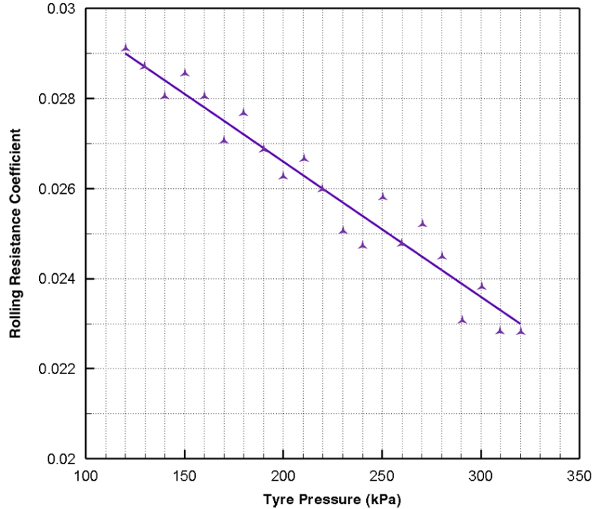
Figure 4: Rolling Resistance Coefficient vs. Tyre Pressure
