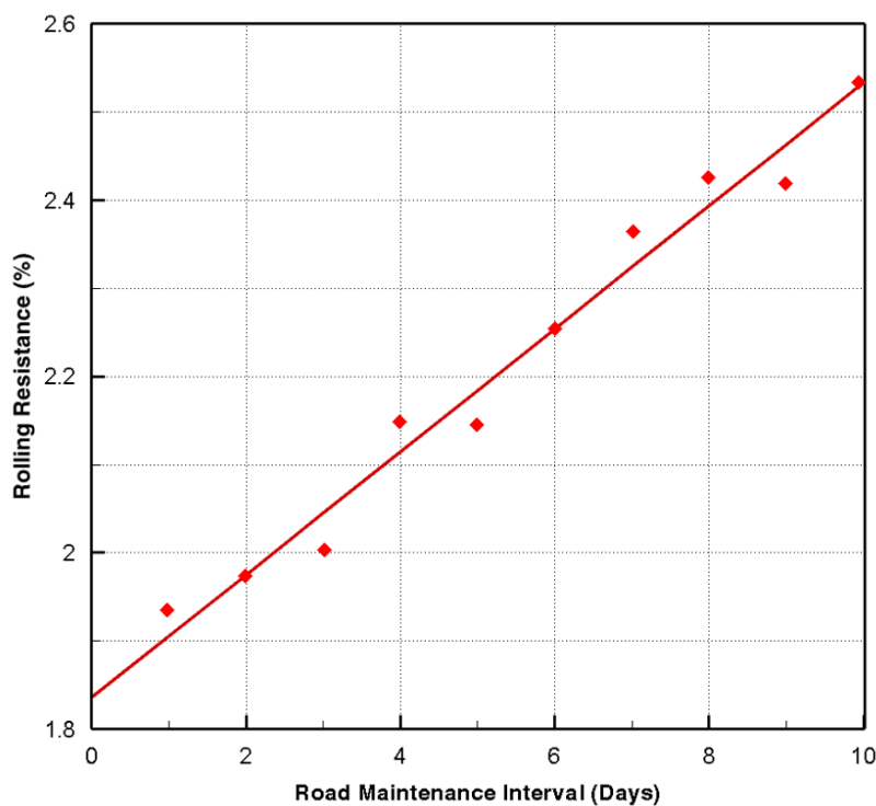
Figure 3: Rolling Resistance vs. Road Maintenance Interval
