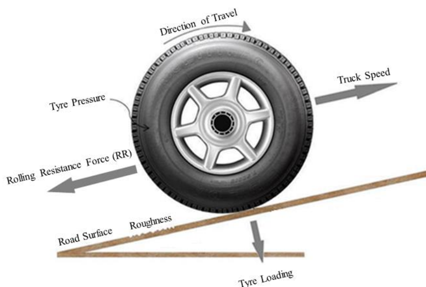
Figure 1: Rolling Resistance and the most Influential Parameters
