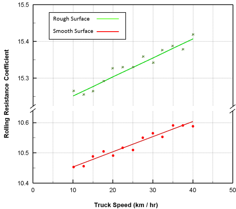
Figure 5: Rolling Resistance Coefficient vs Truck Speed
